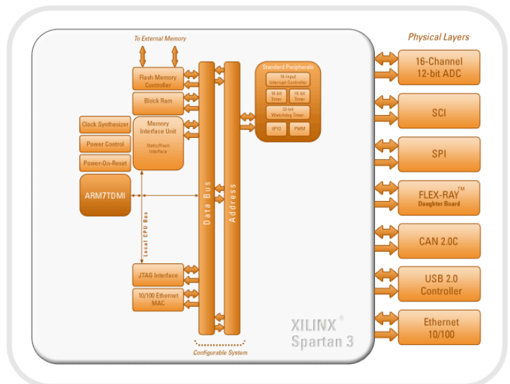
Block Diagram of the Si-Gate X-1500 Field Configurable System-On-Chip
